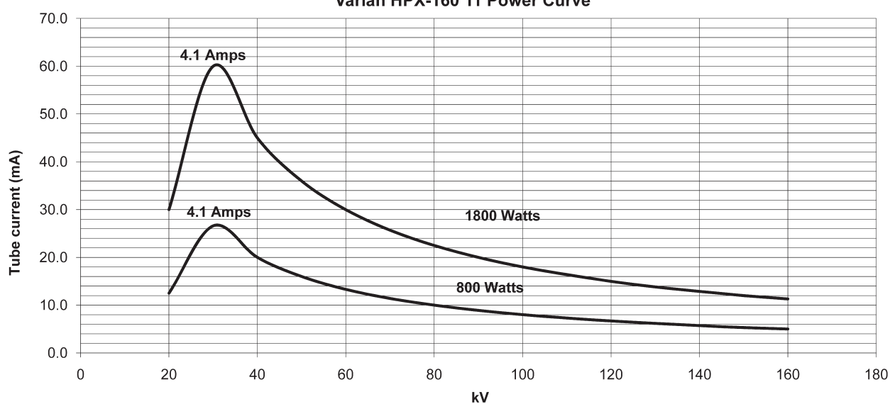
Varian HPX-160 11 Power Curve
