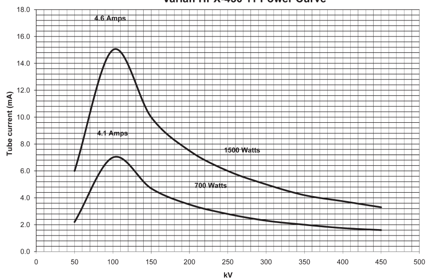
Varian HPX-450 11 Power Curve
