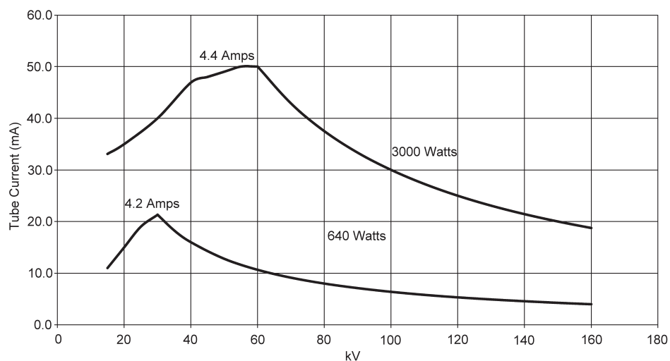
Varian NDI-160-22 Power Curve
