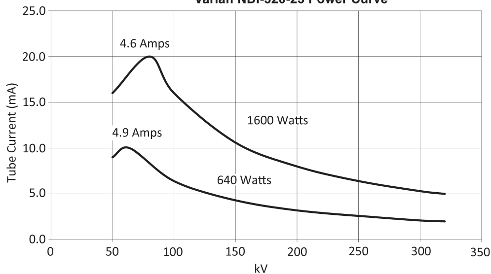
Varian NDI-320-23 Power Curve
