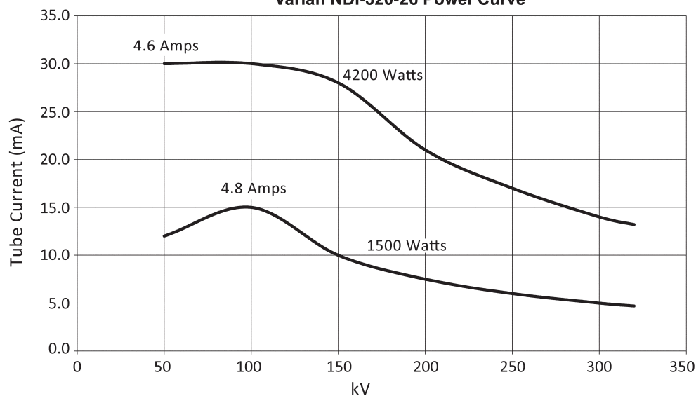
Varian NDI-320-26 Power Curve
